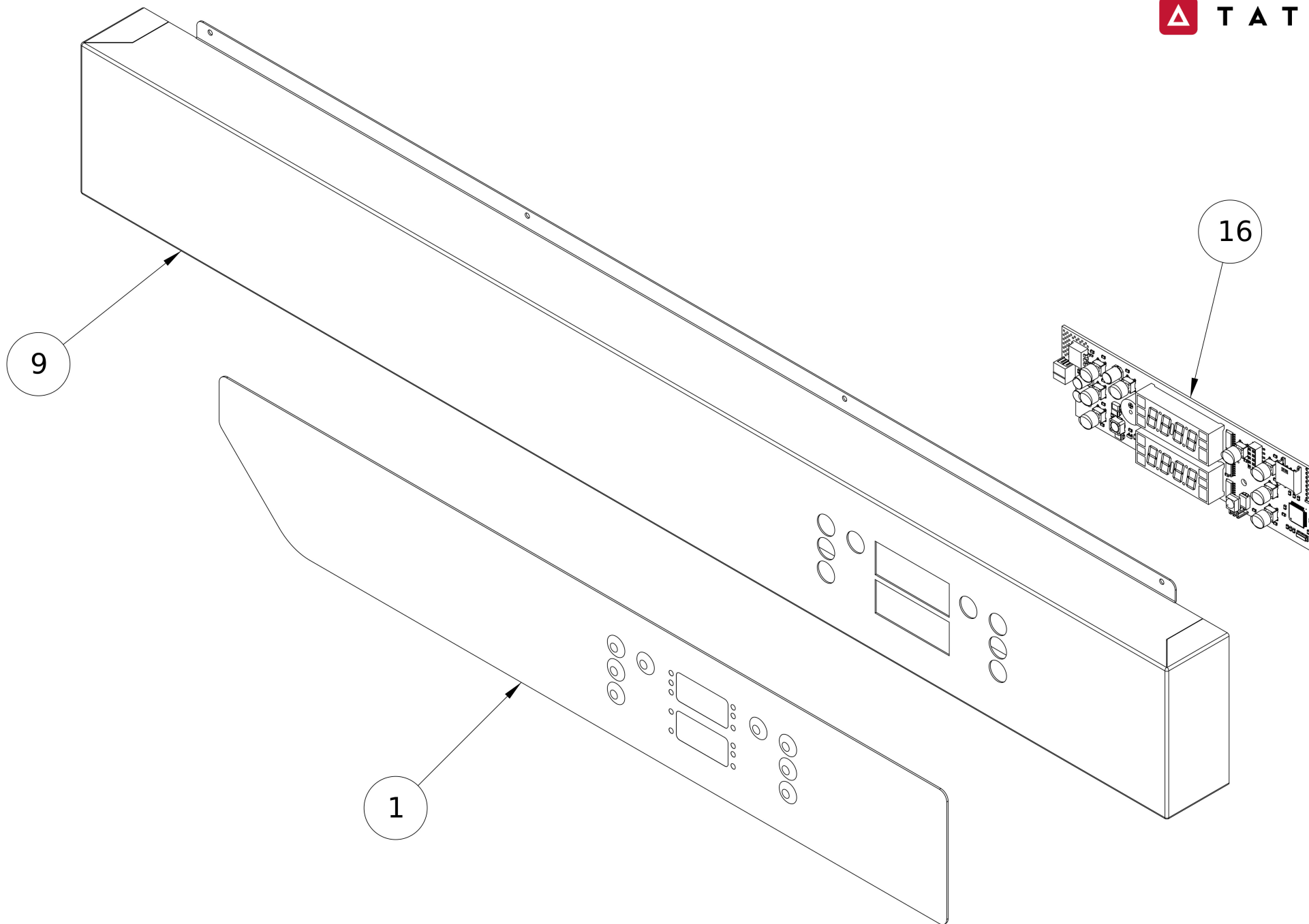
Frontal panel
